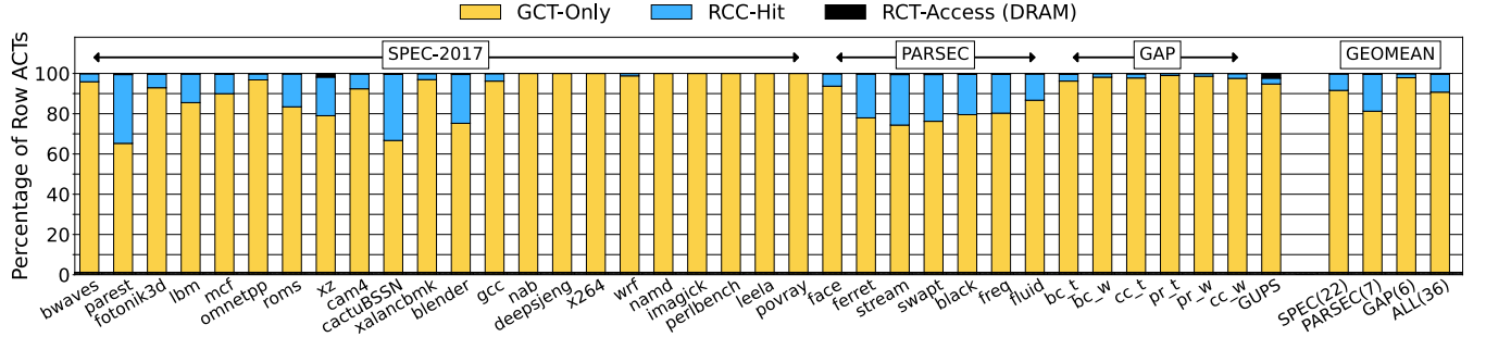
Figure 6: Distribution of activation count updates depending on where they were satisfied in Hydra (a) filtered by GCT (b) hit in the RCC cache (c) serviced by the RCT in DRAM. On average, only 0.3% need to go to the DRAM.
